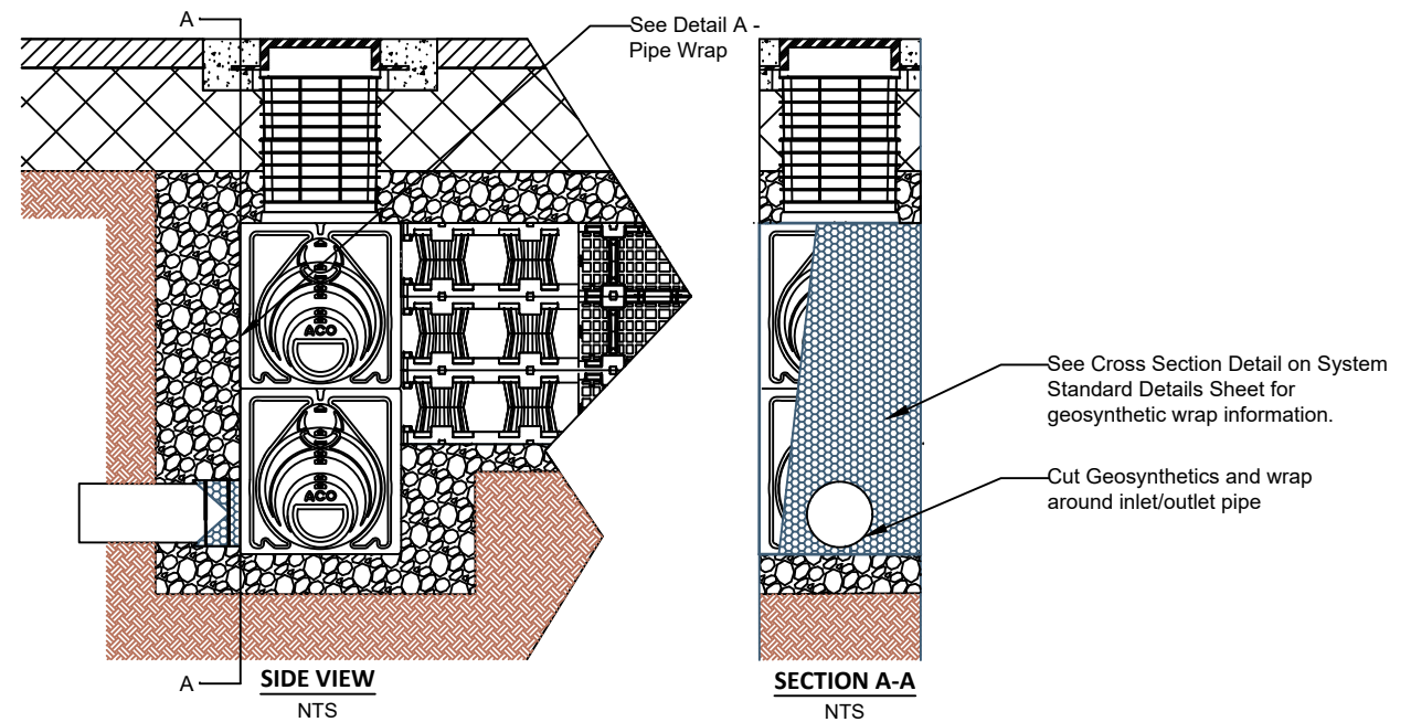
3 LAYER 300HD - REMOTE ACCESS UNIT PIPE INSTALLATION NTS
