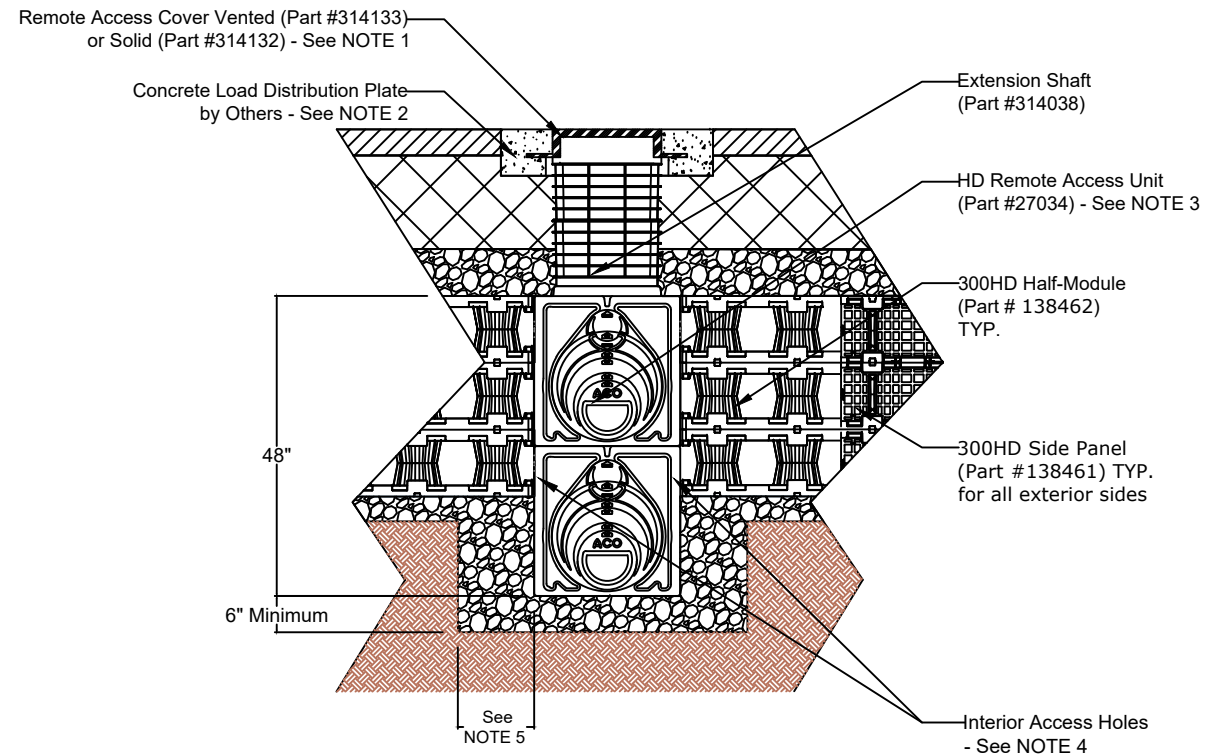
3 LAYER 300HD REMOTE ACCESS UNIT CROSS SECTION NTS
